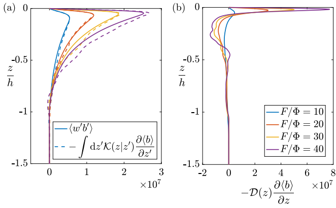
Fig. 7. (a) Comparison of the eddy fluxes \langle w'b' \rangle (solid curve) with the estimate from the kernel -\int dz' \mathcal{K}(z|z') \partial b / \partial z' for four different MLD. (b) An estimate of the flux using the appropriate local diffusivity \mathcal{D}(z) for four different values of MLD. In each case, the MLD is defined as the ratio of the penetrating shortwave heat flux to the diffusive heat flux in the deep thermocline, h = \ln(F/\Phi) .
