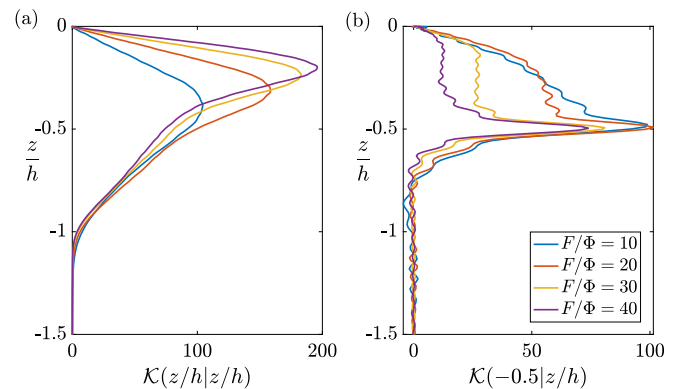
Fig. 6. (a) The diagonal elements of the kernel, showing the local effect of the mixing, plotted against z/h , where h is the MLD, and (b) a horizontal slice of \mathcal{K}(z/h|z'/h) in the middle of the mixed layer at z/h = -0.5 illustrating the non-local effects of mixing for four different values of MLD. In each case, the MLD is defined as the ratio of the penetrating shortwave heat flux to the diffusive heat flux in the deep thermocline, h = \ln(F/\Phi) .
