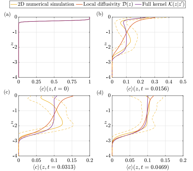
Fig. 9. The time-evolution of a passive tracer added to the flow near the surface, as given by the 2D DNS, and solution to Eqs. (19a) and (19b). The yellow dotted curves represent 1 standard deviation from the mean ensemble profile (yellow curve) obtained by averaging 100 realizations in the 2D DNS. (a) shows the initial profile at t = 0 which is given by Eq. (20) for d = 0.25 . The ratio of the penetrating shortwave heat flux to the diffusive heat flux in the deep thermocline is F/\Phi = 10 .
