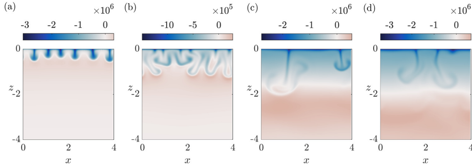
Fig. 1. The panels show the evolution of the deviation of buoyancy field, b(x, z, t) - \Phi z , at four times, t = 0.03, 0.04, 0.49, 1.10 for F/\Phi = 20 .
