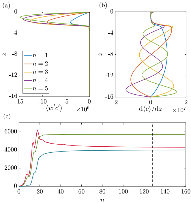
Fig. 3. (a) and (b) show the horizontally averaged eddy fluxes and gradients of tracer concentration corresponding to f_n(z) where n = 1, 2, 3, 4, 5 . (c) Convergence of the kernel \mathcal{K}(z|z') with n in terms of the maximum eigenvalue (multiplied by 100 for scale, green curve), sum of the absolute values of \mathcal{K}(z|z') (red curve), and the sum of the squares of \mathcal{K}(z|z') (blue curve). The vertical line represents n = 128 . Here, the ratio of the penetrating shortwave heat flux to the diffusive heat flux in the deep thermocline is F/\Phi = 10 .
