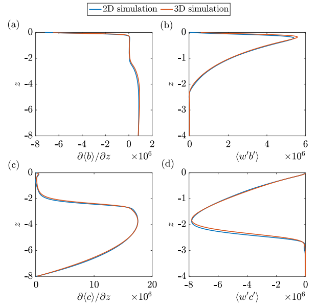
Fig. 8. Comparison of the horizontally averaged fluxes and gradients of buoyancy and passive tracer in 2D and 3D simulations with the same boundary conditions. The 3D simulations are done using a finite volume code (Ramadhan et al., 2020) whereas the 2D simulations use a pseudo-spectral code (Burns et al., 2019). In both sets of simulations, the ratio of the penetrating shortwave heat flux to the diffusive heat flux in the deep thermocline is F/\Phi = 10 , so that the MLD is h = \ln(F/\Phi) \approx 2.3 . The profiles for the passive tracer are estimated by solving Eq. (12) where f(z) is given by Eq. (B.2) for n = 1 .
