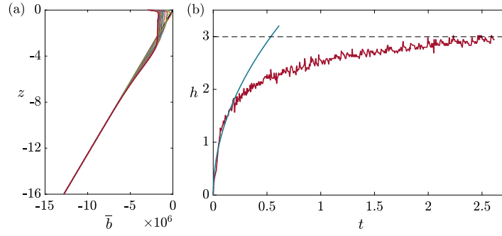
Fig. 2. (a) Horizontally averaged buoyancy \bar{b} plotted at various times as represented by the different colors, starting with a linear profile (black line) at t = 0 . (b) The variation of MLD h versus time t . The horizontal line represents h = \ln(F/\Phi) and the blue curve represents h \sim \sqrt{t} . Here, the ratio of the penetrating shortwave heat flux to the diffusive heat flux in the deep thermocline is F/\Phi = 20 .
