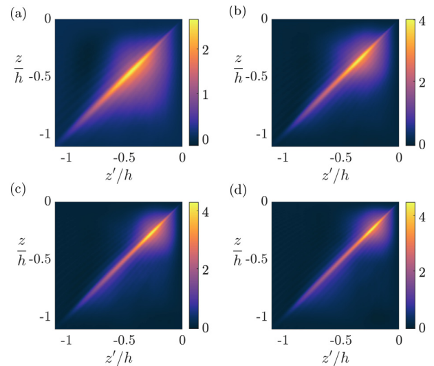
Fig. 5. (a)–(d) show the kernel \mathcal{K}(z/h|z'/h) for four different values of MLD, h = \ln(F/\Phi) , obtained by varying the ratio of the penetrating shortwave heat flux to the diffusive heat flux in the deep thermocline, where F/\Phi = 10, 20, 30, 40 respectively.
