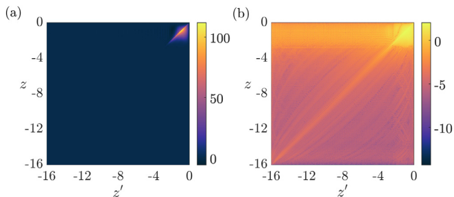
Fig. 4. (a) \mathcal{K}(z|z') . (b) \log_{10}|\mathcal{K}(z|z')| . Here, the ratio of the penetrating shortwave heat flux to the diffusive heat flux in the deep thermocline is F/\Phi = 10 , and the kernel is computed using n = 128 tracers.
