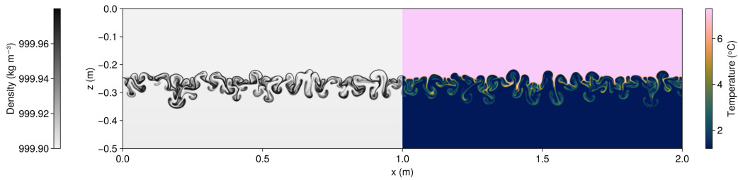
Figure 3: Density and temperature at t = 1 minute in a direct numerical simulation of cabbeling in freshwater. Note that both fields span from x = 0 to x = 2 meters; only the left half of the density field and the right half of the temperature field are shown.
