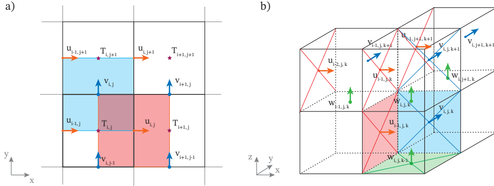
Figure 10: Locations of cell centers and interfaces on a two-dimensional (a) and three-dimensional (b) staggered grid. In (a), the red and blue shaded regions highlight the volumes in the dual u -grid and v -grid, located at (Face, Center, Center) and (Center, Face, Center), respectively. In (b), the shaded regions highlight the facial areas used in the fluxes computations, denoted with \mathcal{A}_x , \mathcal{A}_y , and \mathcal{A}_z .
